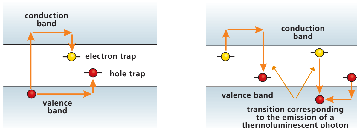
Figure II-12 – Energy levels of a semiconductor material containing impurity
