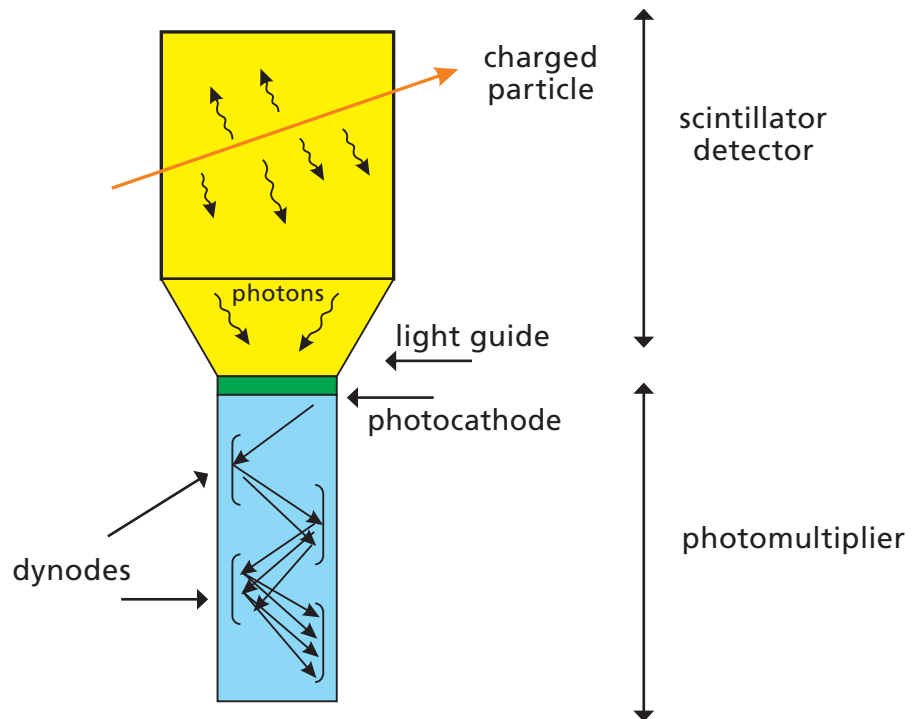
Figure II-10 – Schematic of a scintillator detector, with photomultiplier
