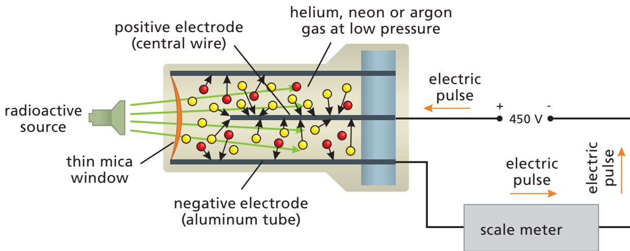
Figure II-9 – Schematic of a Geiger-Muller counter
