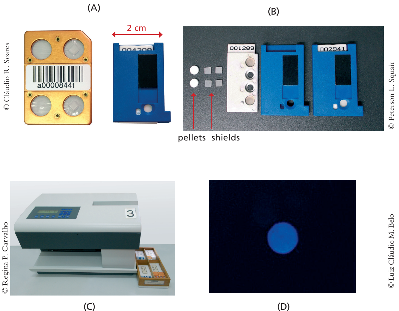
Figure II-11 – Thermoluminescent Detectors (TLDs)
