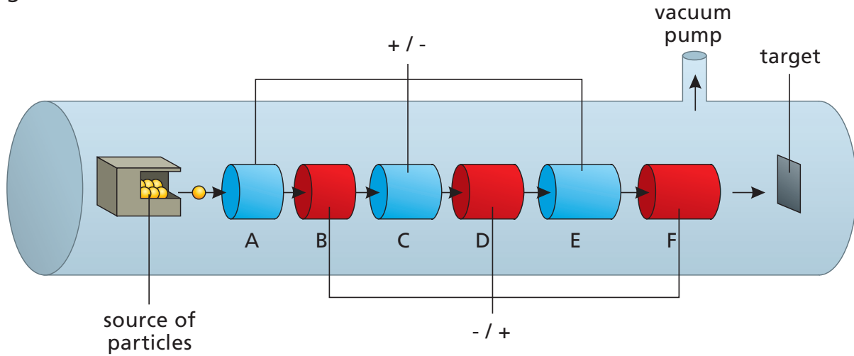
Figure II-1 - Schematic of a linear accelerator
