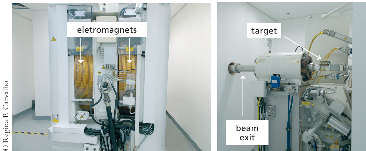
Figure II-3 – Cyclotron (CDTN-CNEN, Brazil)
