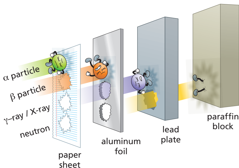
Figure I-1 – Materials that can shield the particles
