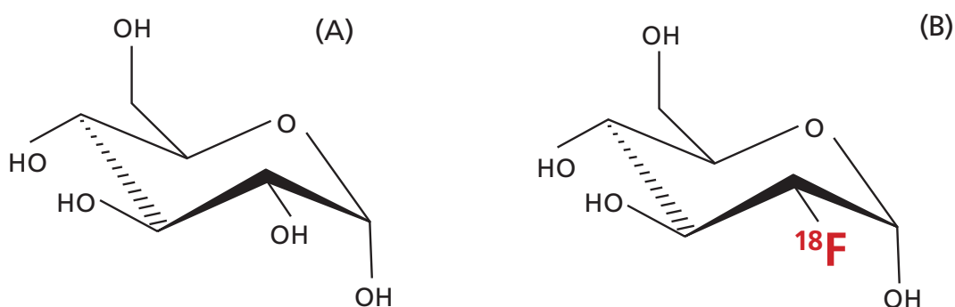
Figure III-2 – Structure of glucose (A) and fluorodeoxyglucose [ ^{18}\text{F} -FDG] (B)
