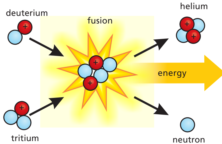
Figure I-5 - Sketch of the fusion reaction
