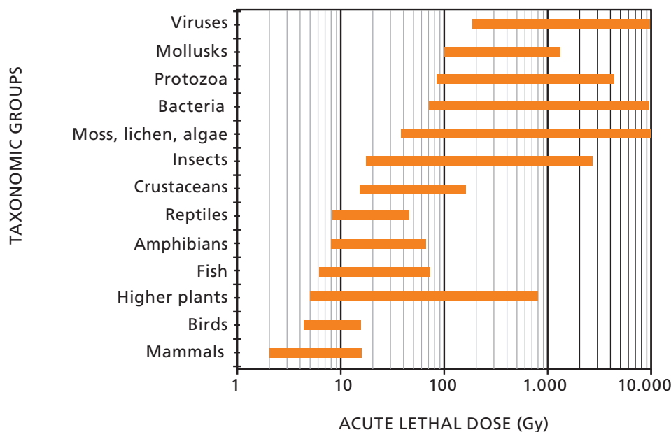
Figure II-8 – Lethal dose of radiation for various living organisms
