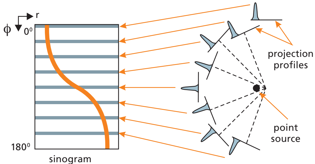
Figure A2-2 – Sinogram obtained based on the projections of a point source, with acquisitions in the range of 0^\circ to 180^\circ
