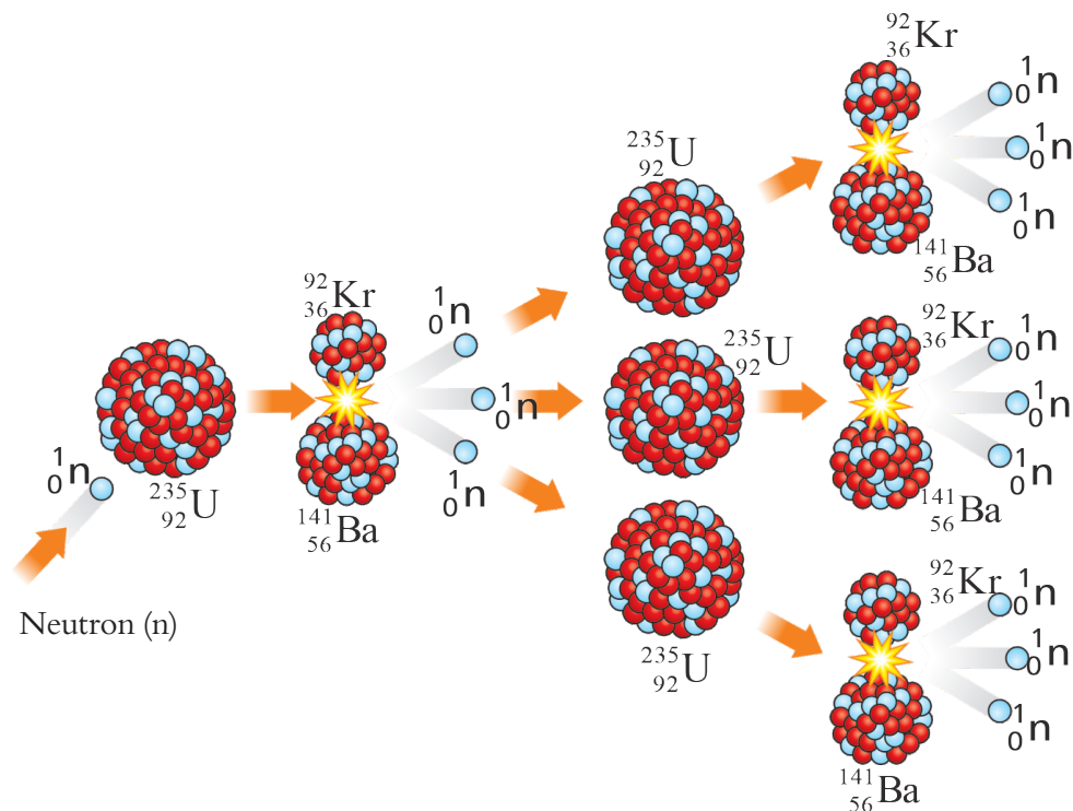
Figure I-4 – Chain reaction in nuclear fission
