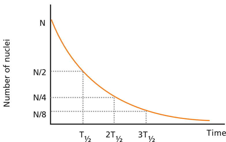
Figure I-2 – Variation in the number of radioactive nuclei as a function of time
