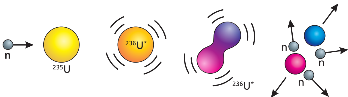
Figure I-3 – A nuclear fission sketch
