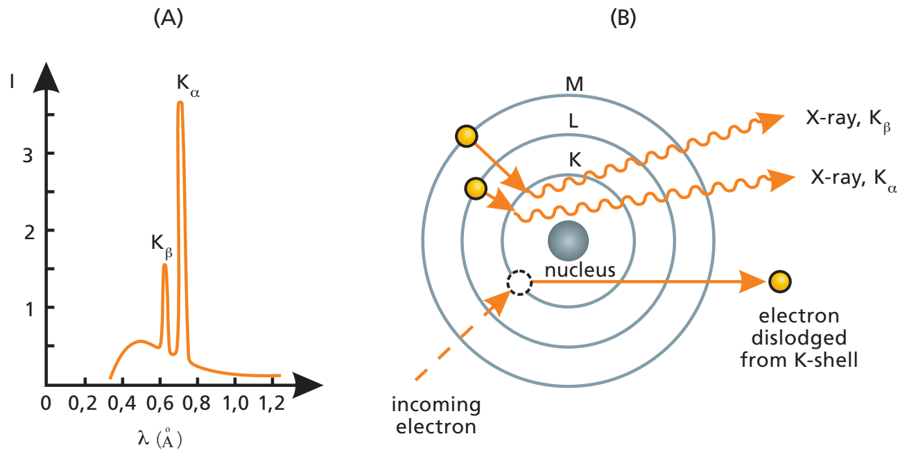
Figure II-4 – X-ray emission by a molybdenum target
