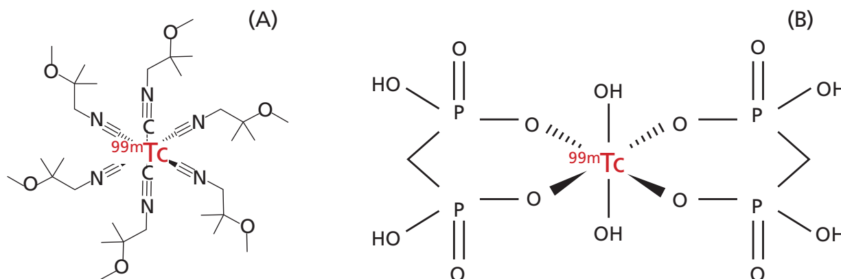
Figure III-1 – ^{99m}\text{Tc} -sestamibi (A) and ^{99m}\text{Tc} -MDP (B)
