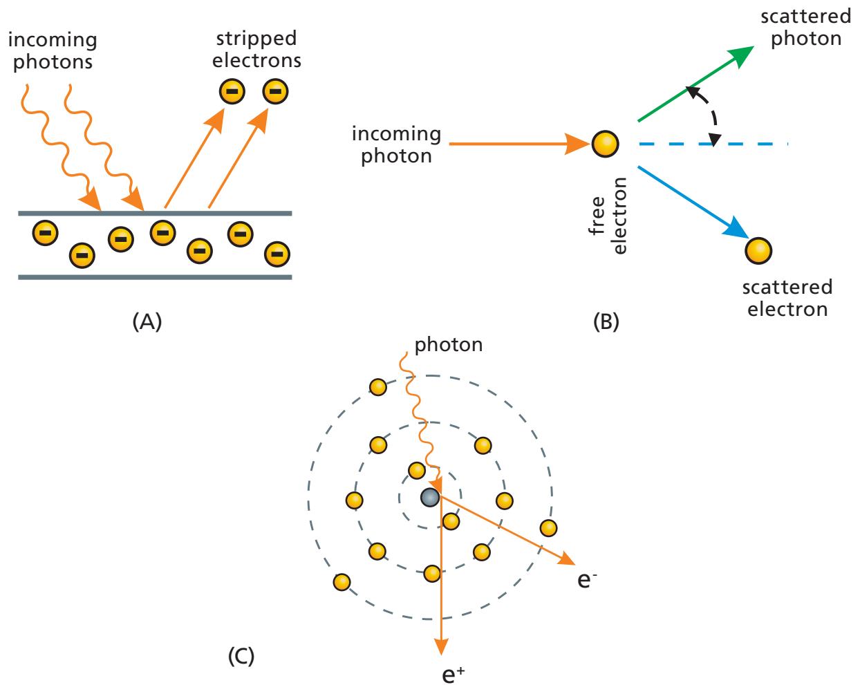
Figure II-5 – Illustration of the photoelectric effect (A) of the Compton effect (B) and pair production (C)
