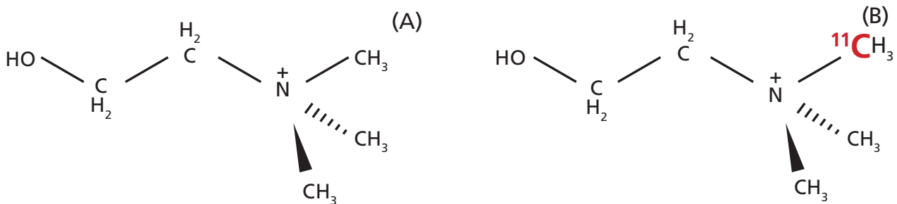
Figure III-3 Structure of the choline
